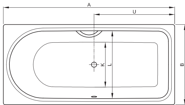
foot end right and overflow front, article no. 8837
