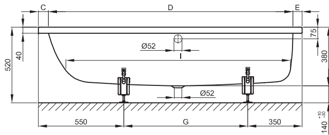
foot end right and overflow rear, article no. 8836
